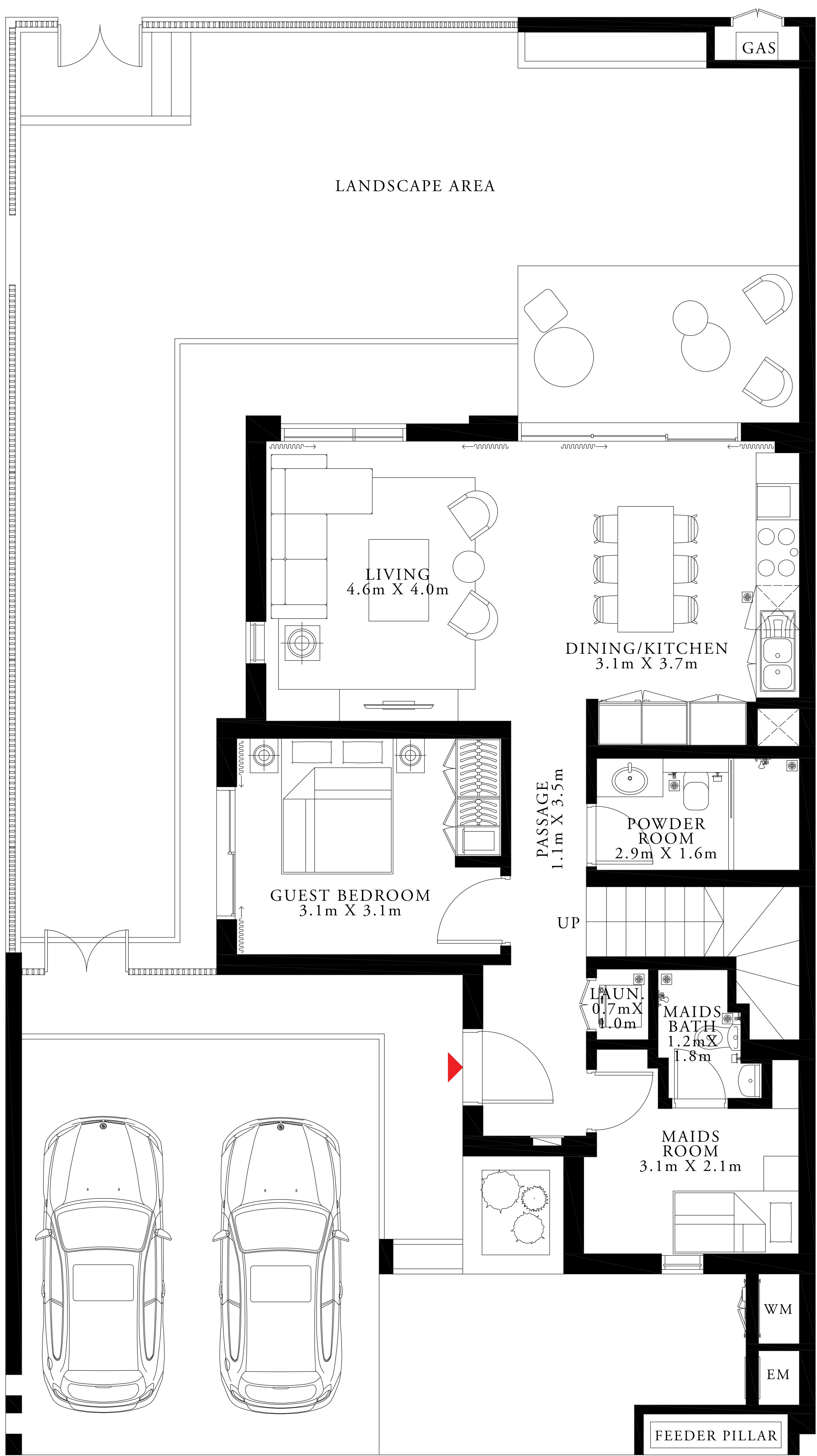
GROUND FLOOR
